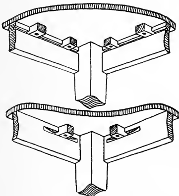
FIG. 425. BUTTONS USED TO FASTEN TABLE TOPS.
